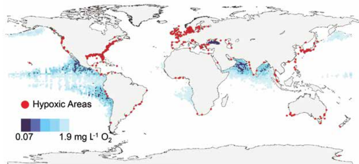
Figure 9.6 Ocean oxygen-minimum zones at 300m depth (blue shaded regions) and coastal hypoxic areas of < 2 \text{ mg O L}^{-1} caused or exacerbated by anthropogenic nutrients (red dots). Figure reproduced with permission from Breitburg et al. (2018) and unpublished data from R. Diaz.
