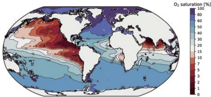
Figure 4.5 Oxygen saturation at the point in the vertical column where oxygen saturation is minimum; computed from the World Ocean Atlas, 2013, version 2 (Garcia et al., 2014). Saturation values less than 15% are coloured in red.
