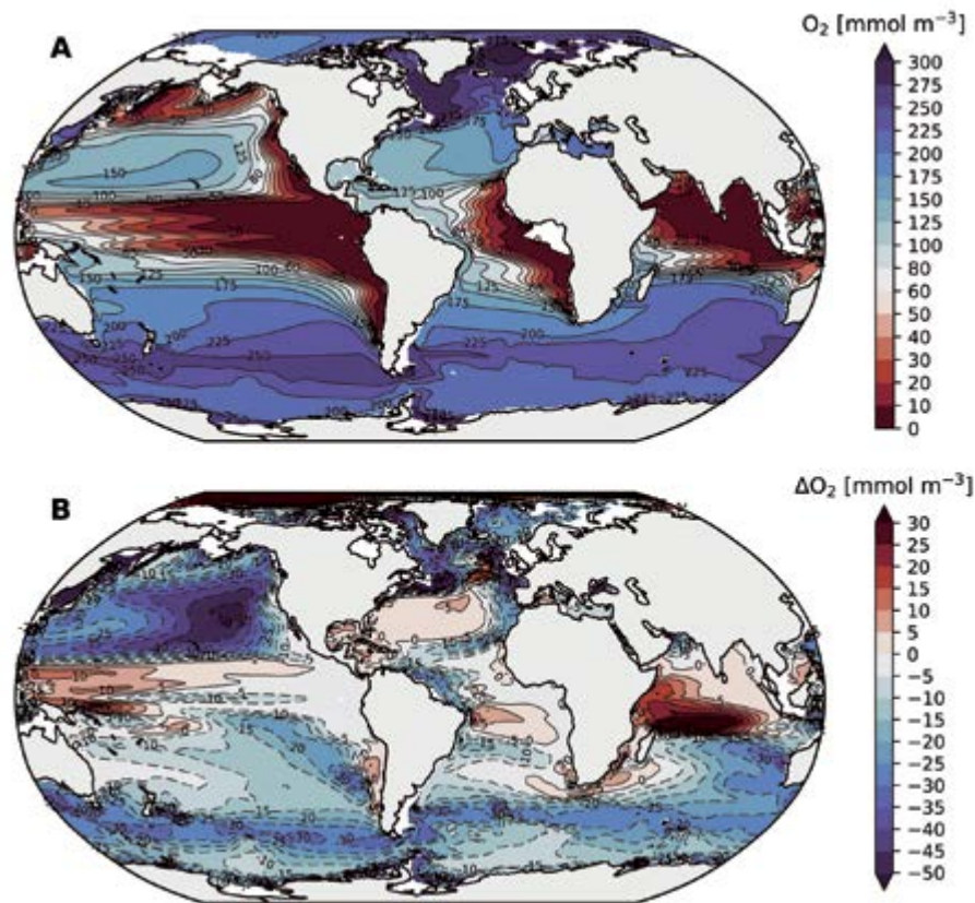
Figure 4.14 Thermocline (mean over the 200–600 m depth range) oxygen distributions simulated by the CESM-LE: (A) O_2 concentration in the control climate; (B) change in O_2 concentration at 2100. The ensemble mean over the period 1920–1939 is used to define the “control” climate.
