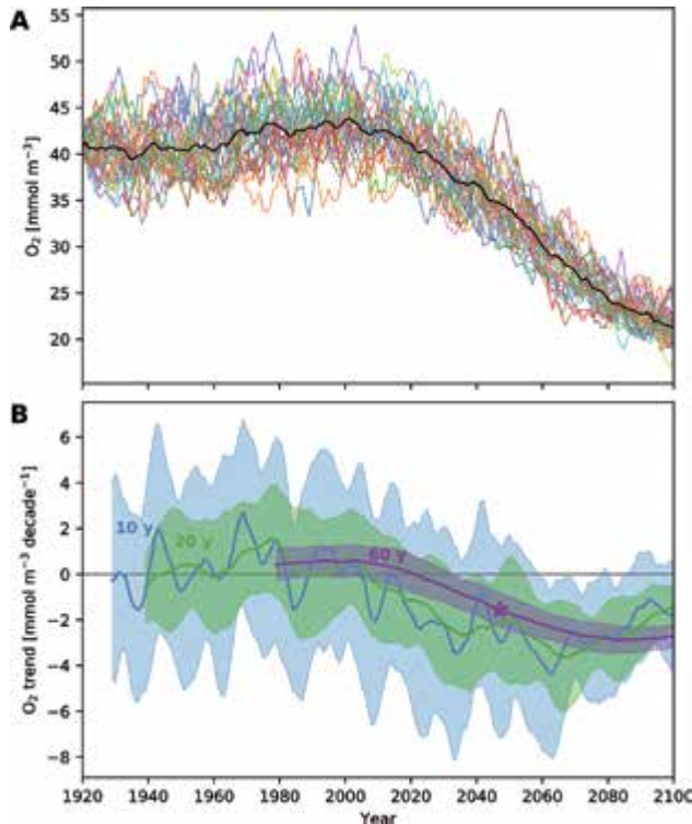
Figure 4.18 Oxygen concentrations and trends in the thermocline of the California Current System (CCS) simulated by the CESM-LE. (A) Oxygen concentrations in the CCS; coloured lines show individual ensemble members, the black line is the ensemble mean. (B) Retrospective trends computed from the data displayed in (A).
