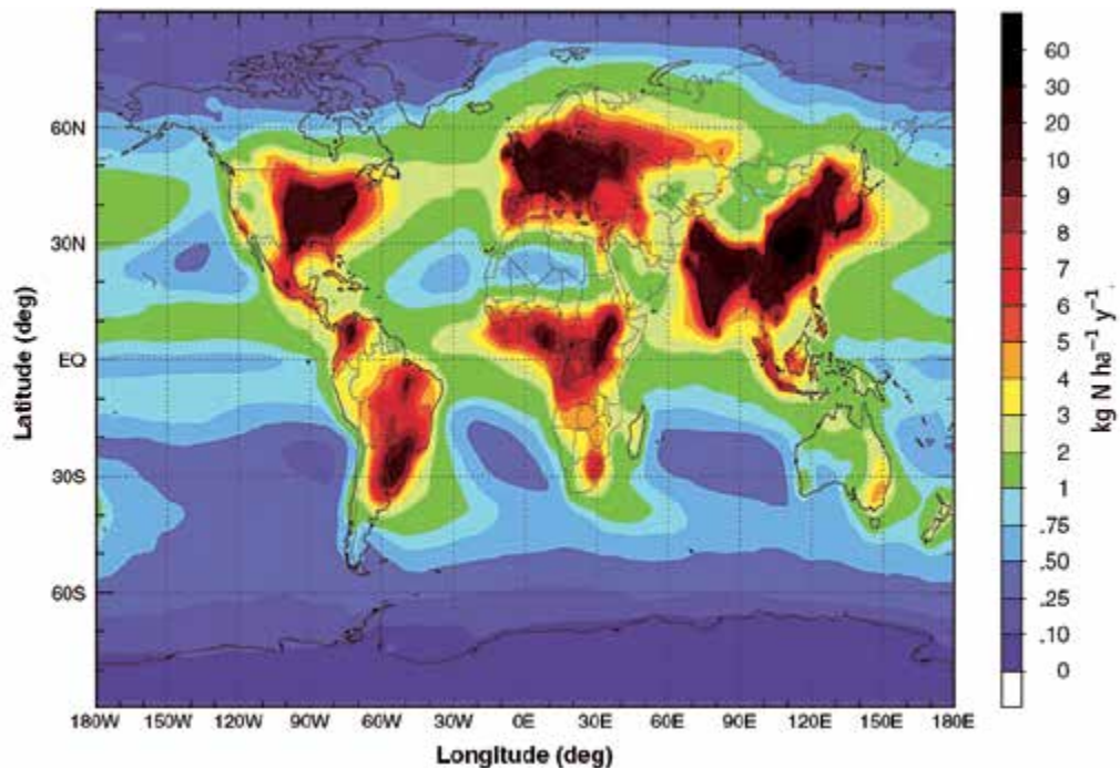
Figure 2.5.2 Global nitrogen deposition estimated from total N ( \text{NO}_y and \text{NH}_x ) emissions, 105 \text{ Tg N yr}^{-1} (Galloway et al., 2008).
