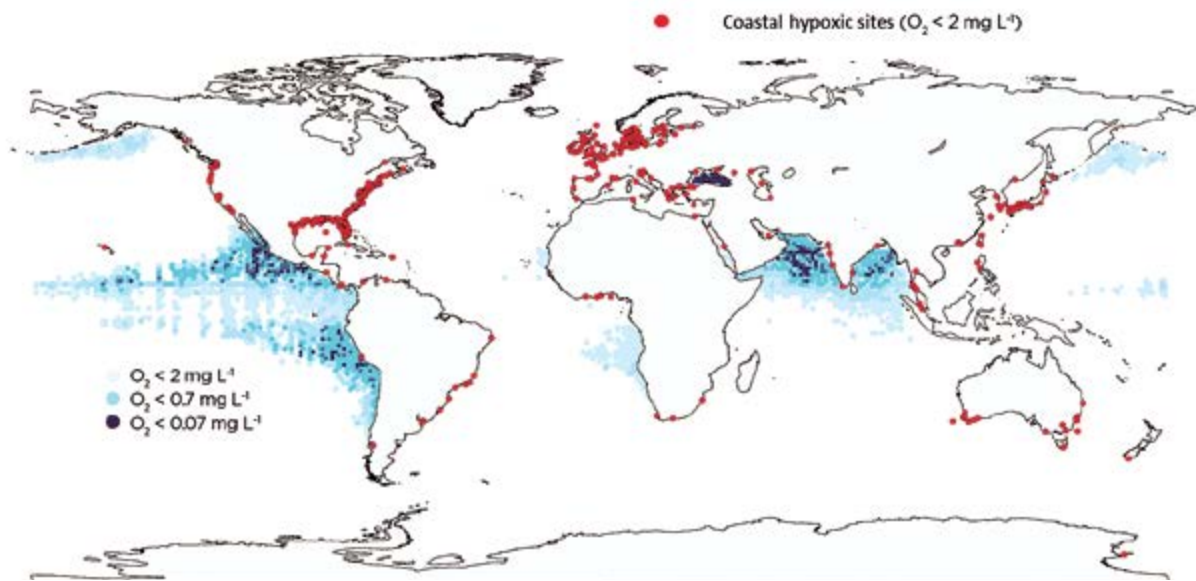
Figure 1.3 Global distribution of deoxygenation in the coastal and global ocean (from Breitburg et al., 2018). In the coastal area, more than 500 sites have been inventoried with low oxygen conditions while in the open ocean the extent of low oxygen waters amounts to several millions \text{km}^3 .
