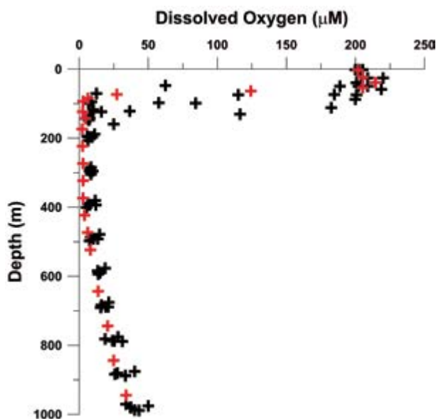
Figure 2.3.8 Comparison of O_2 distribution in the northern Bay of Bengal in the vicinity of Lat. 18^\circ N , Long. 89^\circ E based on sampling in April 1963 (black symbols) and April 2007 (red symbols).
