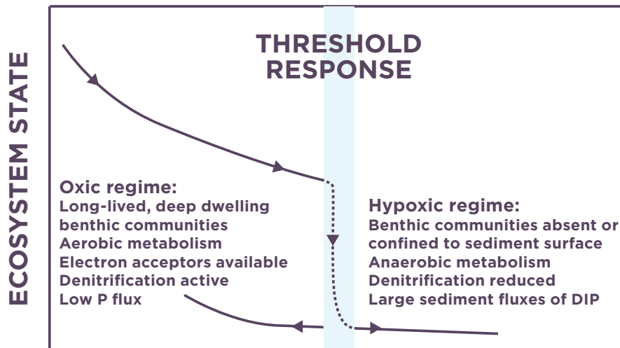
Figure 7.6 Hypothetical diagram showing change in ecosystem state as represented by bottom water oxygen concentrations versus nutrient concentrations. An ecosystem is believed to reach a threshold when bottom-living organisms are killed and the system switches to one dominated by anaerobic processes (Conley et al., 2009a).
