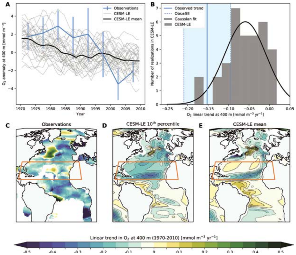
Figure 4.21 O_2 trends in the Subtropical North Atlantic (STNA; 15^{\circ} – 35^{\circ} N) from observations and CESM-LE. (A) STNA average O_2 concentration at 400 m depth from 1970 to 2010. The thin solid lines represent individual ensemble members of the CESM-LE, and the thick solid line is the ensemble mean. The blue line is the pentad time series of objectively mapped O_2 dataset based on the World Ocean Database (Ito et al., 2017). Error bar indicates one standard deviation of the pentad data. (B) Histogram of linear O_2 trend at 400 m. The black line is a gaussian fit, and the blue solid is the observed trend; the dashed lines and shaded region show its uncertainty as measured by one standard error. (C) Observed pattern of linear trend at 400 m depth from 1970 to 2010. The trend is plotted for 1^{\circ} \times 1^{\circ} grid cells within which at least 20-years' of observations are available. (D,E) 10th percentile and ensemble mean trend from the CESM-LE for the same depth and time period. The orange box on the maps shows the region for which time series and trends are presented in panels (A) and (B).
