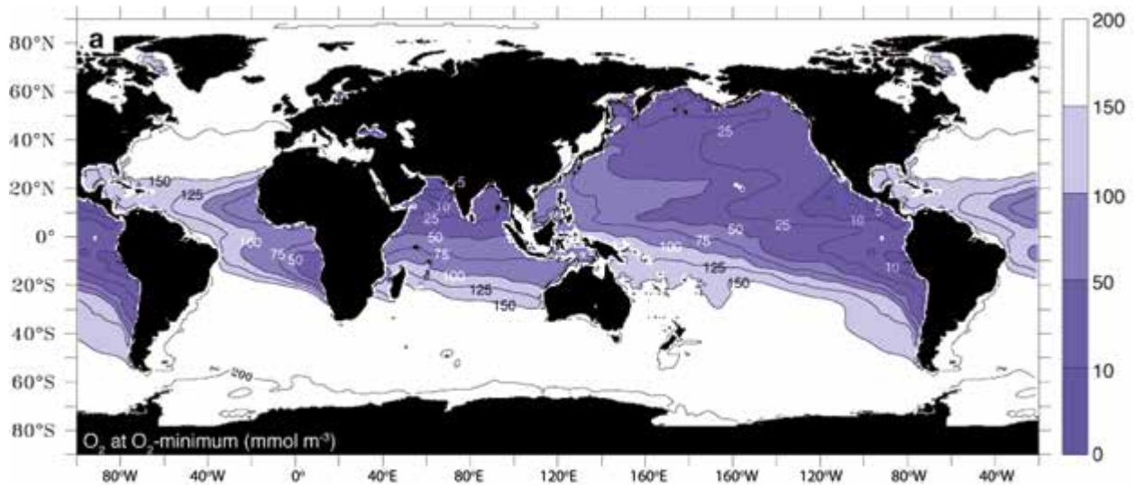
Figure 2.3.2 Distribution of dissolved O_2 ( \mu\text{M} ) at its minimum (after Keeling et al., 2010). The depth of the minimum varies, but in the northern Indian Ocean the lowest O_2 concentrations are generally found below \sim 150 m and above 800 m (Wyrтки, 1971). Note the anomalous location of the oxygen minimum zones in the northern Indian Ocean. Oxygen supply from the south is indicated by the northward tilt of contours along the western boundary (off Africa and Arabia).
