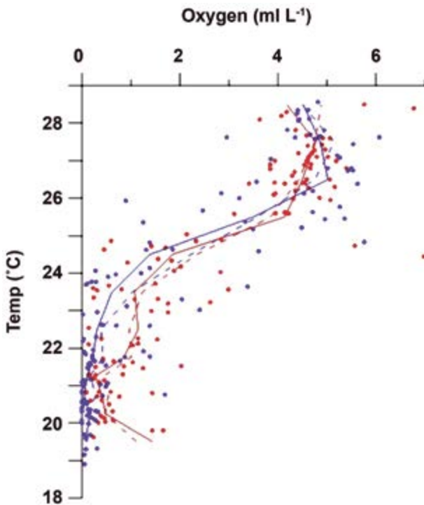
Figure 2.3.10 Comparison of O_2 concentrations with reference to temperatures over the inner and mid-shelf regions (depths < 60 m) off Karwar (see Figure 2.3.1), central west coast of India, during the upwelling period in 1971–1975 (red symbols) and 1997–2004 (blue symbols). Mean and median values for 1 °C-bins are shown by the dashed and solid curves, respectively (modified from Naqvi et al., 2006c).
