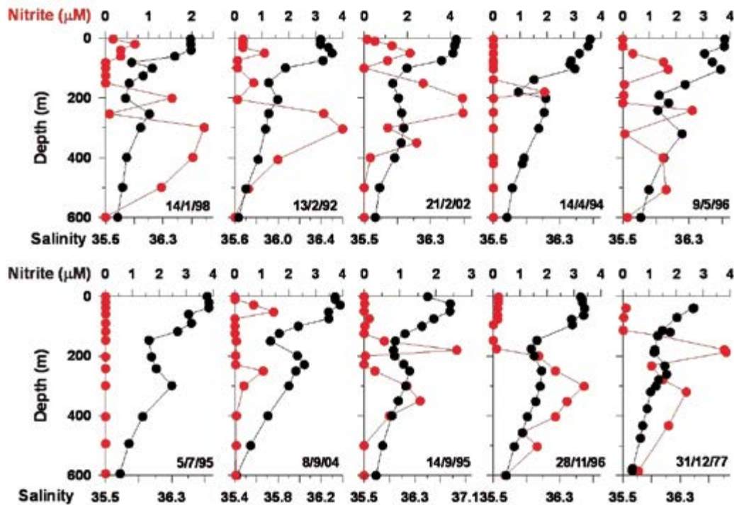
Figure 2.3.6 Vertical profiles of nitrite (red symbols) and salinity (black symbols) at a fixed site (Lat. 19.75°N, Long. 64.62°E) sampled repeatedly between 1977 and 2004 (arranged by month of visit). The station is located close to the north-western boundary of denitrification zone and the observed variability is largely caused by the flow of the high salinity water mass originating in the Persian Gulf (modified from Banse et al., 2014).
