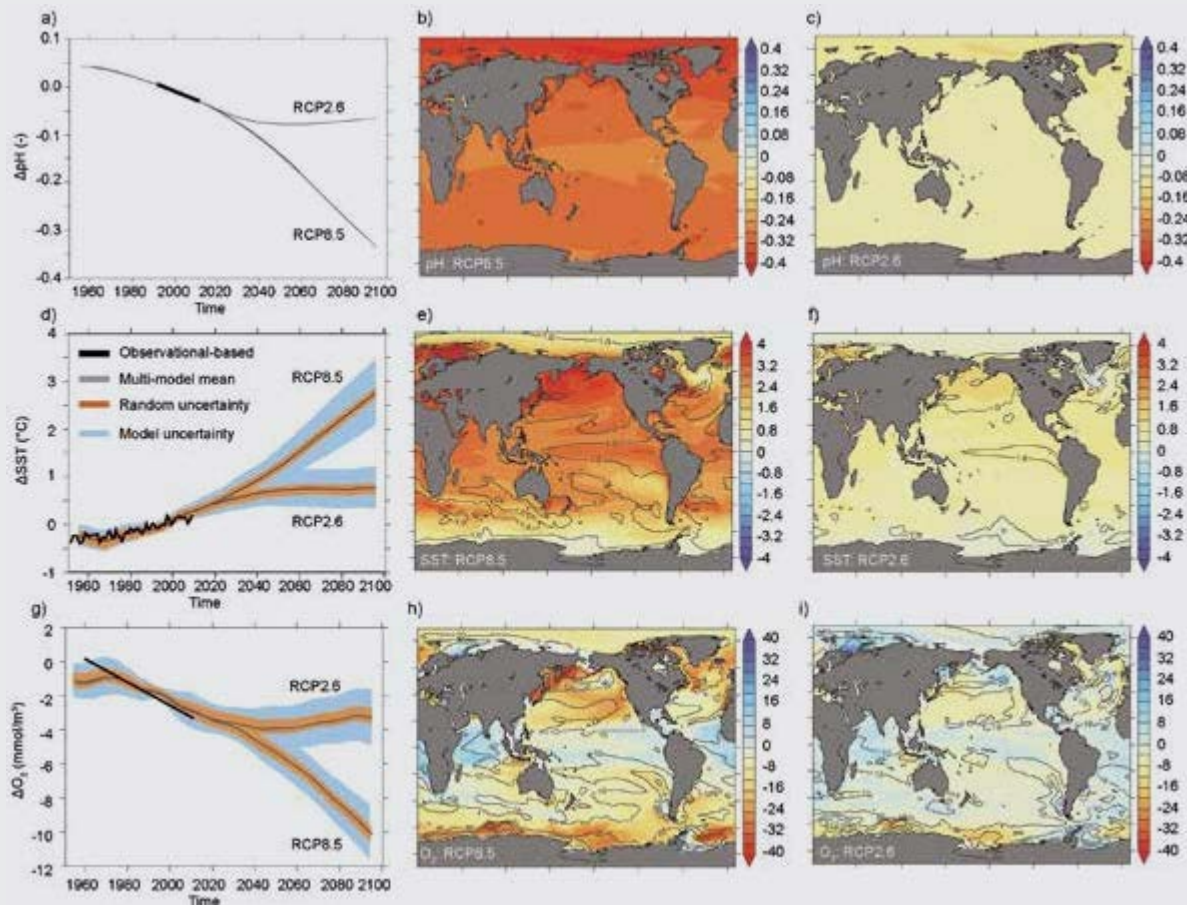
Box Figure 2.1.2 Time series and spatial patterns of simulated change in surface pH, sea surface temperature ( ^\circ\text{C} ), and oxygen concentration ( \text{mmol m}^{-3} ) averaged over 100 to 600 m depth. Simulated spatial patterns of multi-model mean changes in year 2095 for the (middle column) RCP8.5 scenario and right column RCP2.6 scenario (Reprinted with permission from Frölicher et al., 2016 (© Wiley and Sons)).
