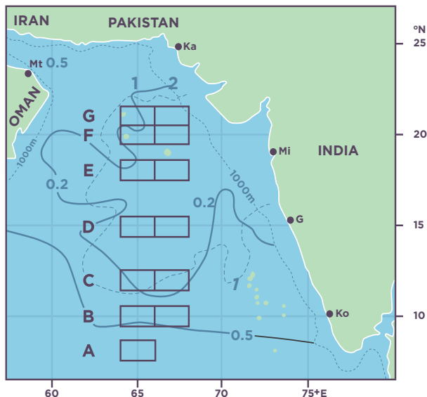
Figure 2.3.5 "Boxes" selected by Barse et al. (2014) to investigate decadal changes within the oxygen minimum zone of the Arabian Sea. The left boxes are numbered "1" while the right boxes are numbered "2". Oxygen distribution at 200 m is shown by the 0.2 and 0.5 \text{mL l}^{-1} contours (solid) from Wyrski (1971); the zone of denitrification is demarcated by the 1 \mu\text{M} nitrite contour (dashed) from Naqvi (1991).
