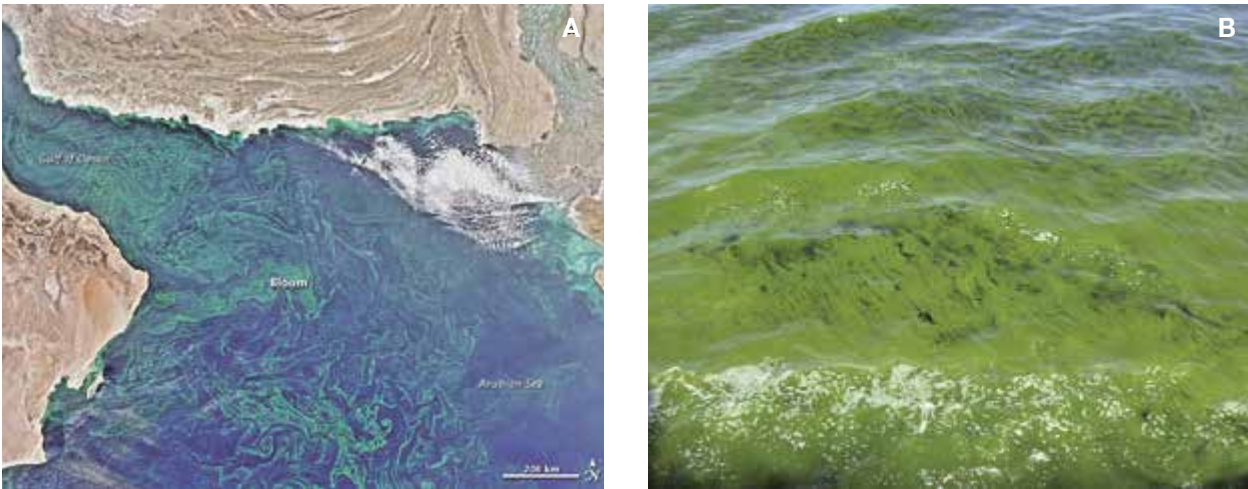
Figure 2.3.7 A) Convective mixing in winter leads to the development of phytoplankton blooms in the northern Arabian Sea, which are identifiable by satellite-based ocean colour measurements. Source: Image obtained on 14.02.2015 by the Moderate Resolution Imaging Spectrometer (MODIS) on NASA's Aqua satellite ( https://earthobservatory.nasa.gov/images/85718/winter-blooms-in-the-Arabian-Sea ). Earlier algal blooms in this region largely comprised diatoms, the major group of phytoplankton with glassy shells. Diatoms were grazed by copepods that were, in turn, eaten by fish. B) Replacement of diatoms by larger sized dinoflagellates ( Noctiluca scintillans bloom in February 2009 (from http://helgagomes.com )), attributed to incursions of low O_2 waters into the surface layer (Gomes et al., 2014), may disrupt this important food chain. Instead the photosynthesized organic matter may now end up as 'useless' salps and jellyfish with potentially large socio-economic consequences.
