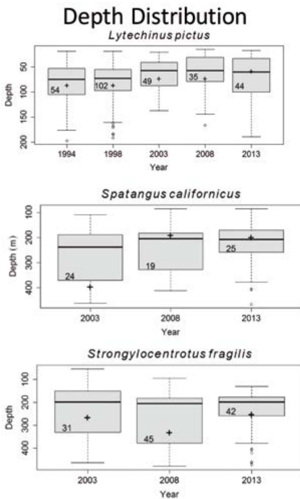
Figure 8.5.6 Changes in sea urchin distribution along the southern California Bight shelf and slope over the past 15-25 years as reported in Sato et al. (2017), based on data from the Southern California Coastal Water Research Project trawl surveys. Oxygen has declined by 20-30% at depths of 200-300 m (Bograd et al., 2014).
