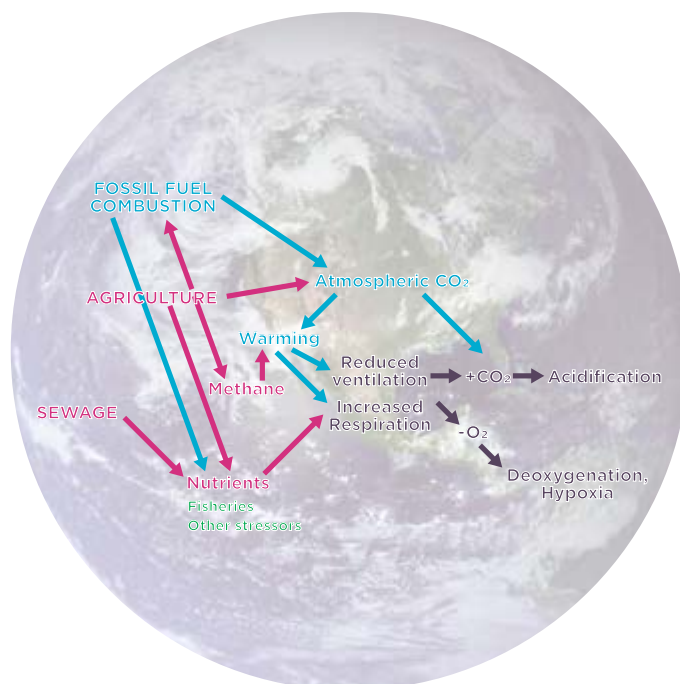
Figure 6.2 Global warming, acidification and deoxygenation are linked. Increasing carbon dioxide in the Earth's atmosphere results in higher ocean temperatures, more acidic conditions, and deoxygenation (Gattuso et al., 2015; Gruber et al., 2012). The warming caused by greenhouse gases, including \text{CO}_2 , lowers oxygen solubility in sea water, increases respiration rates of organisms, and reduces mixing that could otherwise increase exchanges between subsurface waters and the oxygen-rich atmosphere. Respiration by microbes, plants, and animals depletes oxygen and produces \text{CO}_2 , causing further acidification. Nutrients increase total respiration (the biological demand for oxygen) in water bodies by increasing the total production of organic biomass. There are also important feedbacks not illustrated in this figure. For example, extreme low oxygen and anoxic environments can release phosphorus bound to sediment, fuelling further primary production, and are also the sites of production of potent greenhouse gases. Red = major pathways for nutrient sources and effects; blue = major pathways for warming and \text{CO}_2 enrichment; green = other stressors that can increase respiration, for example by altering food webs. (Note that the size of arrows does not indicate the relative importance of these processes.) Earth image: NASA.
